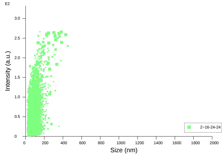
Intensity / Size graph for Experiment: 2 2018-02-27 16-22-15
